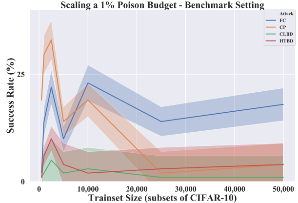
Figure 4. Scaling the dataset size in the benchmark setting.
