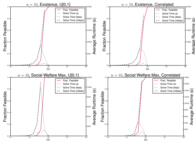
Figure 1: Phase transition for n = 10 under either UNIFORM or CORRELATED, with or without maximizing social welfare.
