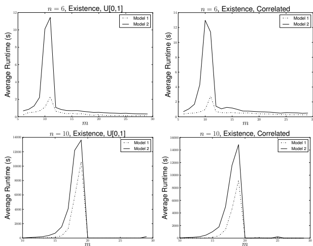
Figure 3: Runtime comparison of Model #1 (feasibility) and Model #2 (optimization) for n = 6 and n = 10 agents.
